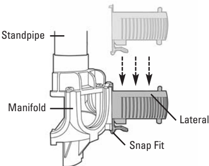
FIGURE 1 - Snap-Fit Detail
