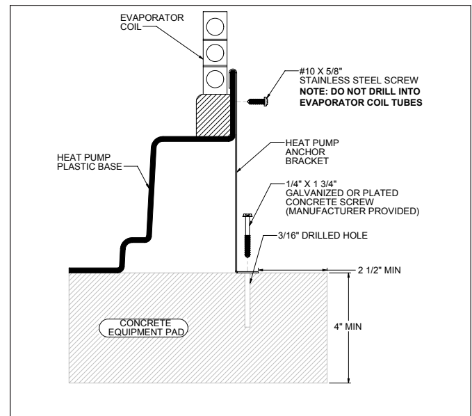
Figure 3. Anchor Clamp Installation
